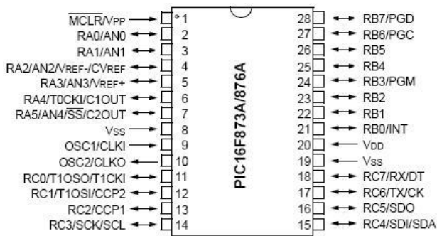
FIGURA 2. PIC 16F876A
